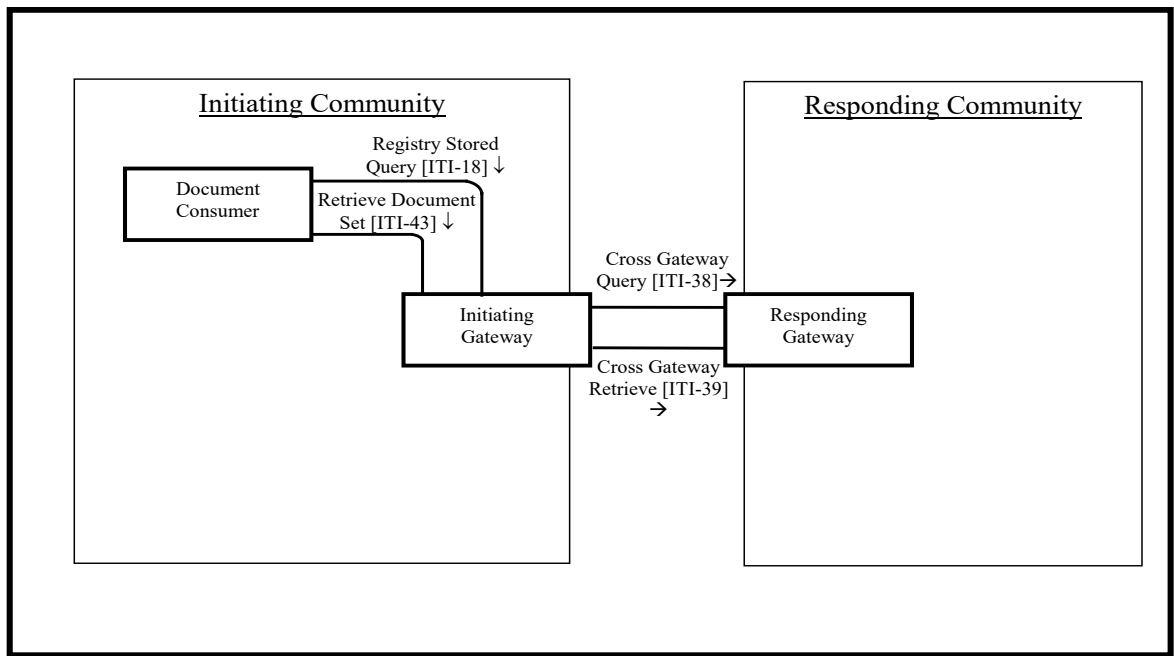
Figure 18.1-1: XCA Actor Diagram
