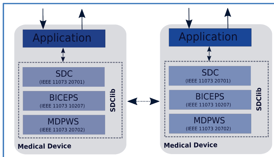
Figure 42 SDC Library - MDPWS Connectivity 85
